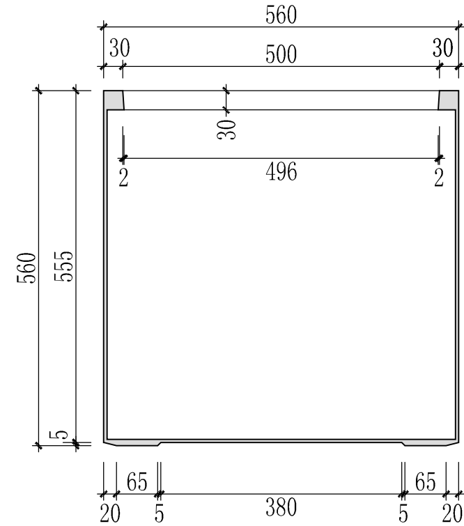
Cross-section
